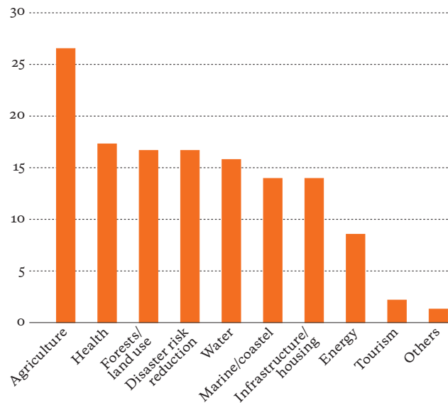
Figure 6: Adaptation priority areas in NAPs (number of mentions) Source: Own analysis of NAPs, June 2016
