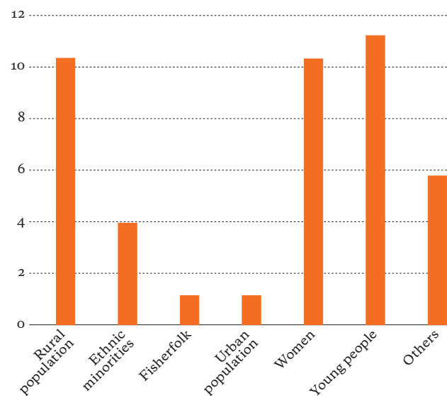
Figure 7: Most climate vulnerable population groups according to NAPs (number of mentions) Source: Own analysis of NAPs, June 2016
