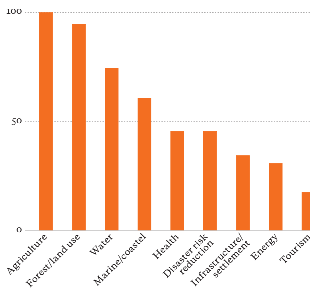
Figure 2: Adaptation priority areas in NDCs (number of mentions) Source: Own analysis of NDCs, July 2016
